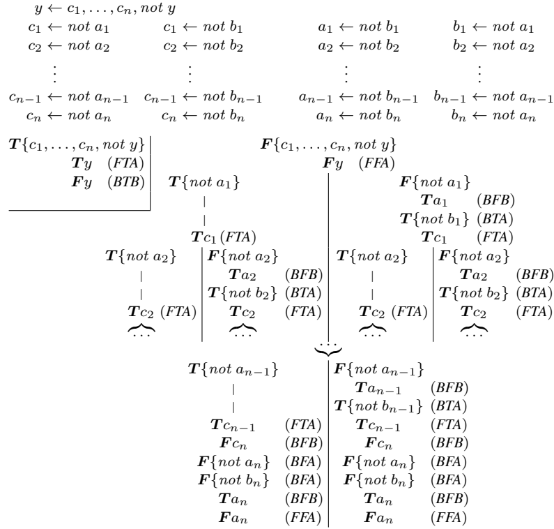
Fig. 12. A minimal refutation of \mathcal{T}_{\text{nomore}} for \Pi_b^n \cup \Pi_c^n , using \text{Cut}[\text{body}(\Pi_b^n \cup \Pi_c^n)] .
