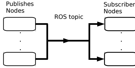
Fig. 1: ROS topics provide many-to-many asynchronous message passing.
